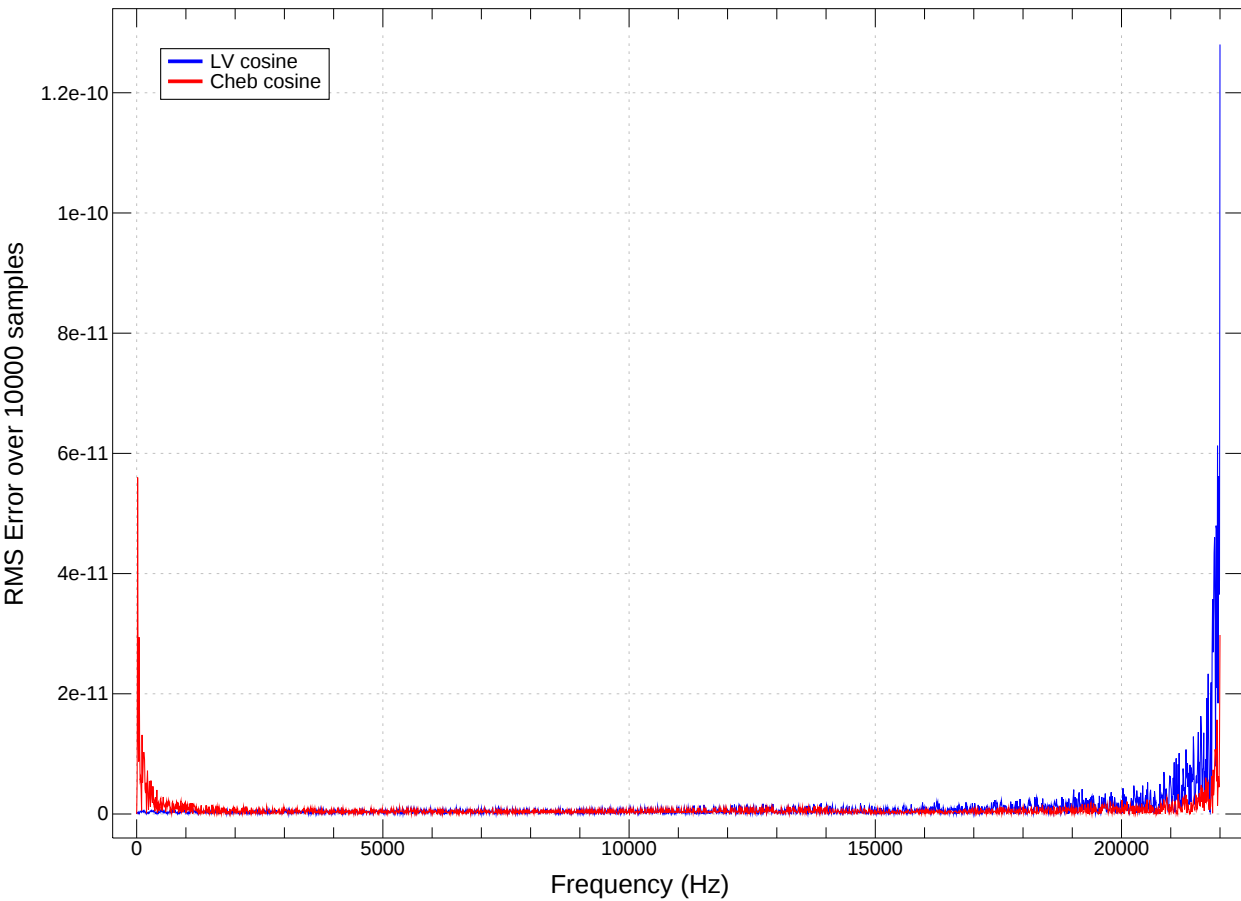
Trig RMS Error vs Frequency
